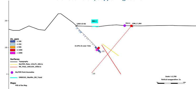
Hole 1393-15-02 | Supporting section
