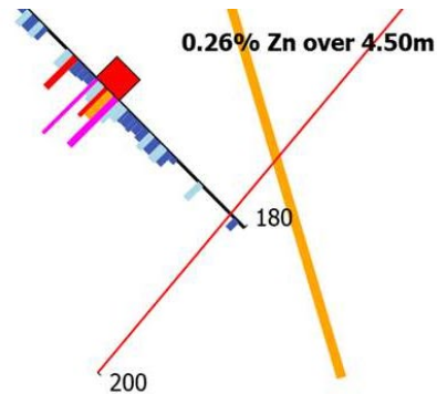
Actual cross-section | Historical holes and modelled conductor geometry
